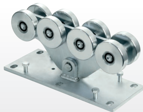
8 wheels cantilever carriage for gates
